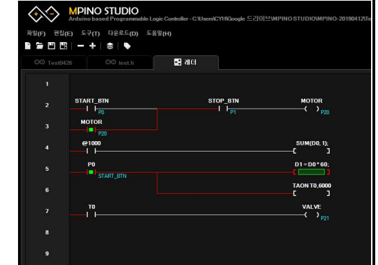
[ LADDER LOGIC ]
